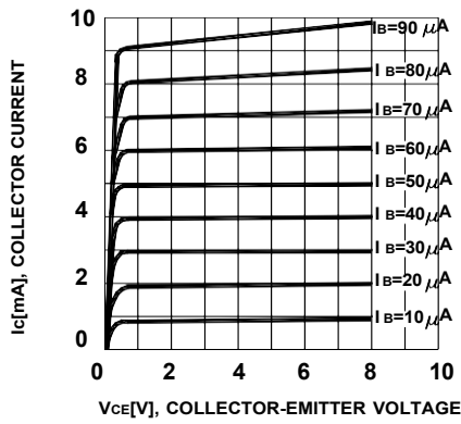
Figure 1. Static Characteristic
