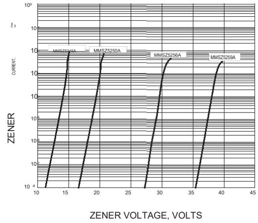
Fig.8 ZENER VOLTAGE VERSUS ZENER CURRENT
