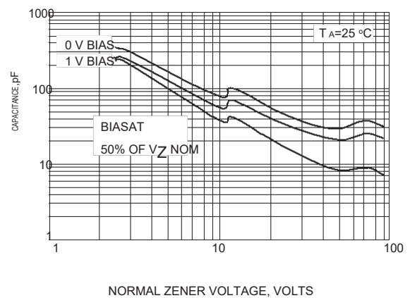
Fig.6 TYPICAL CAPACITANCE
