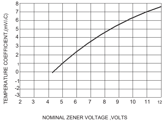
Fig.1 TEMPERATURE COEFFICIENTS
