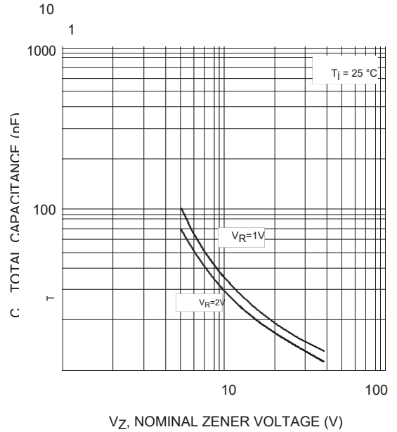
Fig. 2 Total Capacitance vs Nominal Zener Voltage
