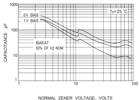
Fig.6 TYPICAL CAPACITANCE
