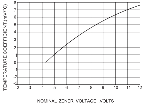
Fig.1 TEMPERATURE COEFFICIENTS
