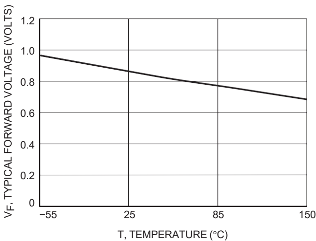
Figure 7. Forward Voltage
