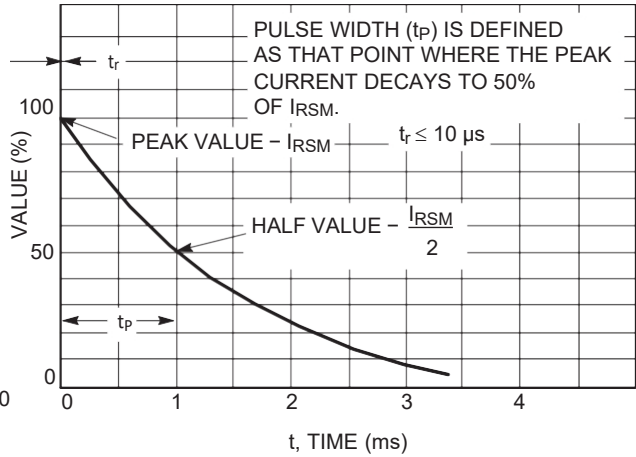
Figure 2. 10 X 1000 μs Pulse Waveform
